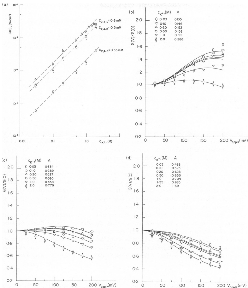
FIGURE 5 (a) Dependence of 2,4-D enhanced nonactin- K^+ conductance on potassium ion concentration in PC-chol membranes. c_{\text{nonactin}} (aqueous solution) = 4.5 \times 10^{-8} M, c_{\text{nonactin}} (membrane solution) = 1.4 \times 10^{-5} M, pH = 2 (buffered), ionic strength (LiCl + KCl) = 2 M. (b-d) Effect of potassium ion concentration on voltage dependence of normalized membrane conductance of PC-chol membranes at three concentrations of 2,4-D. The solid curves were obtained according to Eq. 5 and represent the prediction of the transport model. c_{\text{nonactin}} (aqueous solution) = 4.5 \times 10^{-8} M, c_{\text{nonactin}} (membrane solution) = 1.4 \times 10^{-5} M, pH = 2 (buffered), ionic strength (LiCl + KCl) = 2 M. (b) c_{2,4-D} = 0.35 mM; (c) c_{2,4-D} = 0.50 mM; (d) c_{2,4-D} = 0.60 mM.
