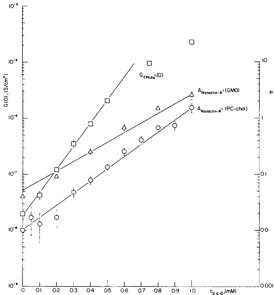
FIGURE 7 A comparison of 2,4-D concentration dependence of TPhAs^+ conductance with that of kinetic parameter A \propto k_{iso}/k_D for PC-chol and GMO membranes. Experimental conditions: PC-chol membranes: c_{TPhAs^+} = 2 \times 10^{-3} M, in c_{LiCl} = 0.5 M. c_{nonactin} (aqueous solution) = 1.1 \times 10^{-7} M, c_{nonactin} (membrane solution) = 3.2 \times 10^{-5} M, c_{K^+} = 0.06 M, ionic strength (LiCl + KCl) = 1 M, pH = 2 (buffered).
