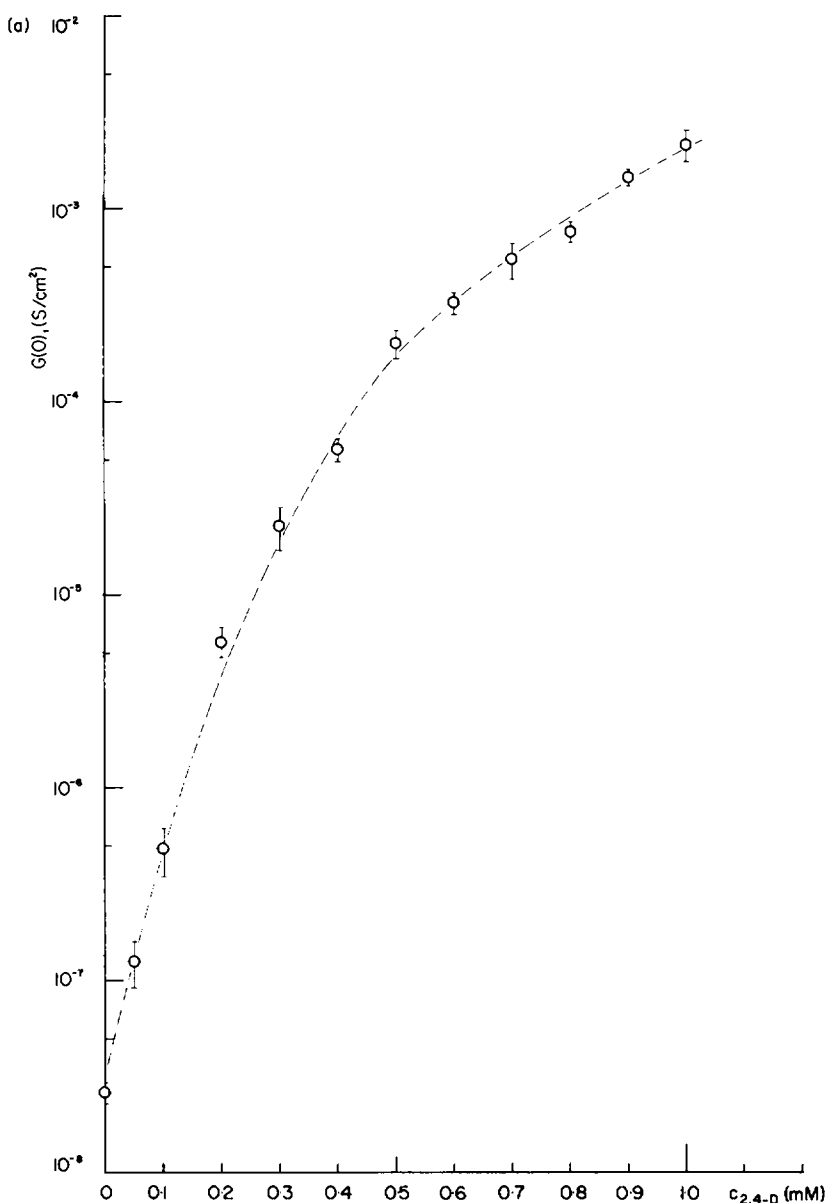
FIGURE 3 (a) 2,4-D enhancement of nonactin- K^+ conductance of PC-chol membranes. Semilog plot of the 2,4-D concentration dependence of zero voltage conductance. Experimental conditions: c_{\text{nonactin}} (aqueous solution) = 1 \times 10^{-7} M, c_{\text{nonactin}} (membrane solution) = 3 \times 10^{-5} M, c_{K^+} = 0.06 M, ionic strength (LiCl + KCl) = 1 M, pH = 2 (buffered). (b) Voltage dependence of 2,4-D enhanced conductance. Plot of normalized membrane conductance G(V)/G(0) versus V as a function of 2,4-D concentration. Each set of data points in this figure corresponds to one conductance point in Fig. 3 a. The solid curves were obtained from Eq. 5 and represent the prediction of the transport model. Experimental conditions: c_{\text{nonactin}} (aqueous solution) = 1 \times 10^{-7} M, c_{\text{nonactin}} (membrane solution) = 3 \times 10^{-5} M, c_{K^+} = 0.06 M, ionic strength (LiCl + KCl) = 1 M, pH = 2 (buffered).
